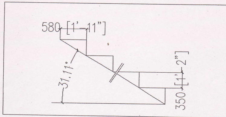
Figure 6.4 :A step chute of length 35m
