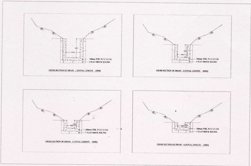
Figure 8.7 : Typical crosssection of proposed drains of various dimensions.
