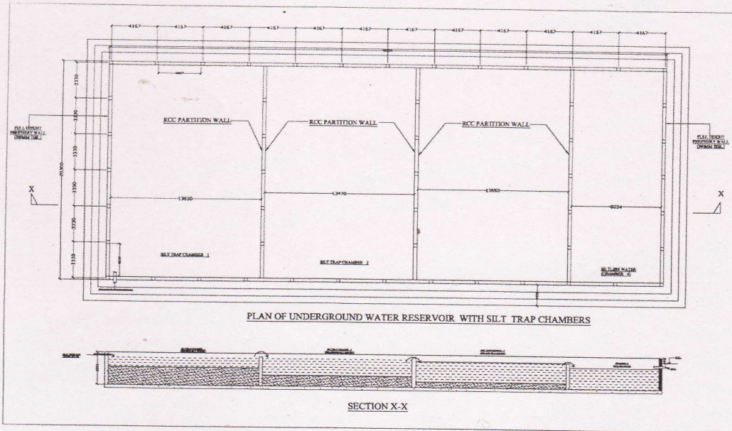
Figure 8.6: Plan of water reservoir including silt traps
