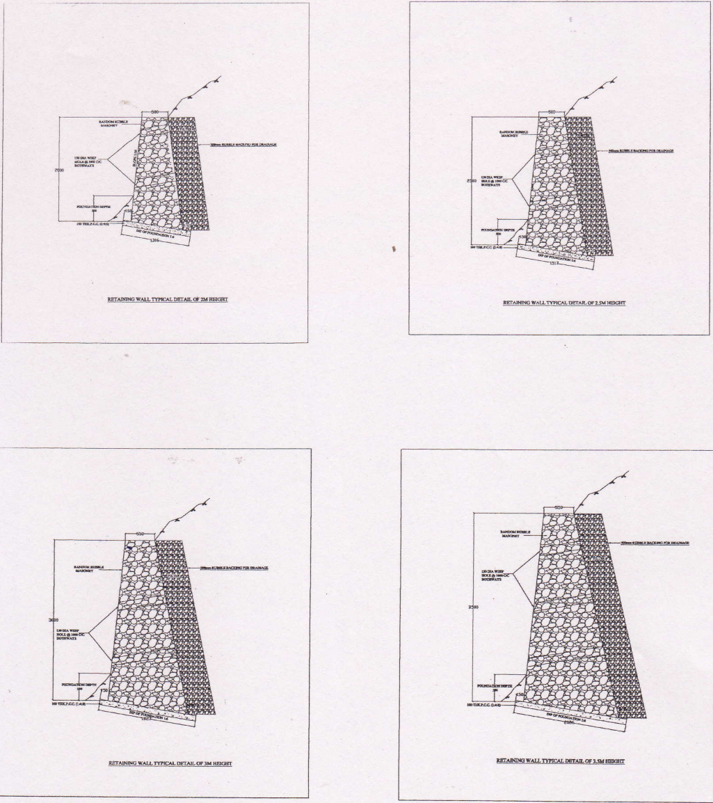
Figure 8.8 : Typical drawing of proposed retaining walls
